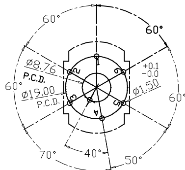
SOLDER SIDE
